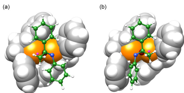
Figure 1. Transition-state structures TS-S (a) and TS-R (b) for hydride insertion of cationic [(R)-Ph-BPE](hydrido)nickel(II) into a \pi -bound N-phenylketimine to give the major (S) and minor (R) isomers, respectively (see Scheme 6a). The ligand Ph-BPE is shown in space-filling mode while other molecules are shown as ball-and-stick models. Nickel is shown in dark red, hydride in pink, phosphorus in orange, nitrogen in blue, and carbon atoms of the ketimine in green.
