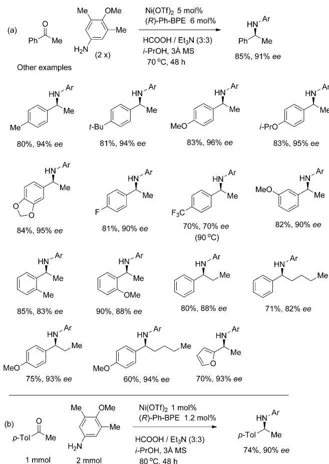
Scheme 3. Asymmetric reductive amination of aromatic ketones with 3,5-dimethylaniline (0.3 mmol scale in most cases).
